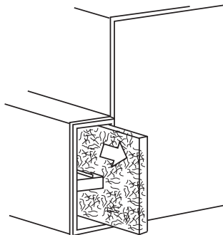
Fig. 16 – Slide Side Filter Out of Furnace
